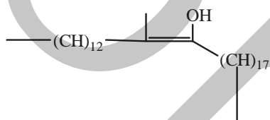
153 14-Methyltriacont-14-en-15-ol
